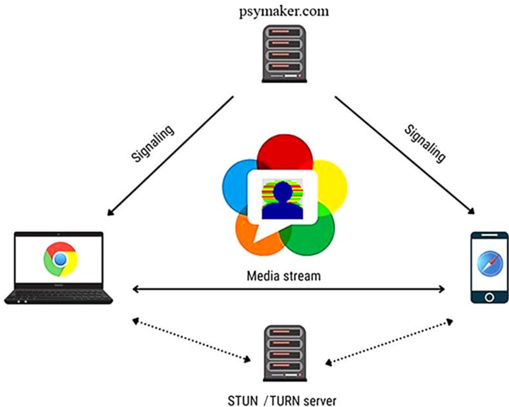
Fig. 4. Block diagram of VibraMed+ program using STUN/TURN servers and Psymaker signaling server to set up optimal peer-to-peer (P2P) communication between the master computer (Doctor) and Internet devices (Patient)
