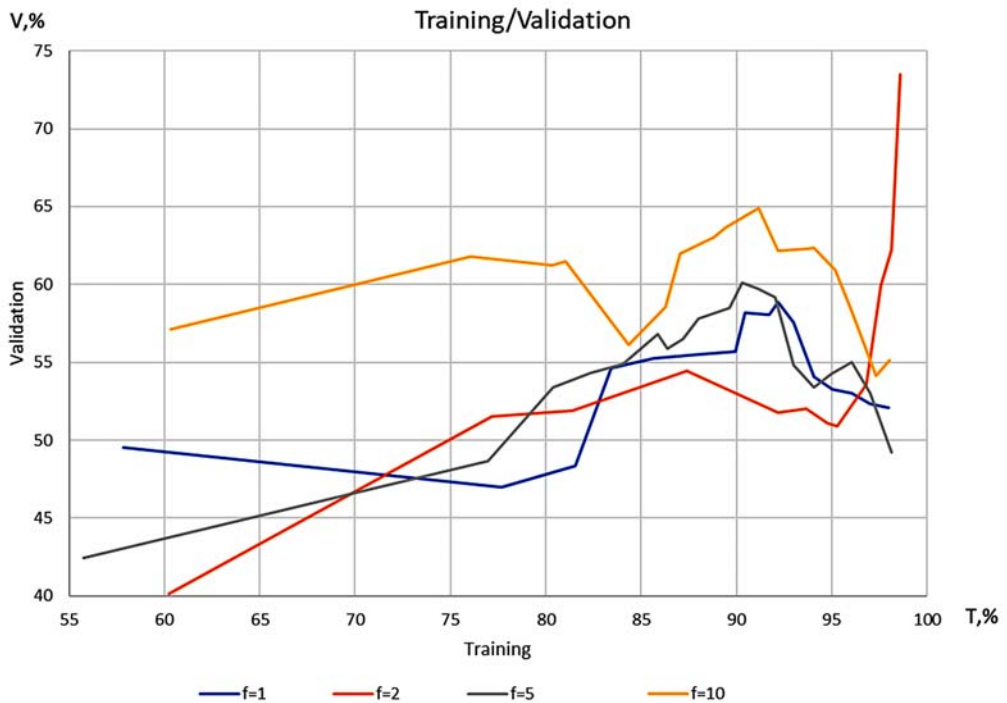
Fig. 2. Measurement accuracy dependences during ANN training of validation database (V, %) on the discrimination accuracy of training database (T, %) for different sampling rates ( f=1, 2, 5, 10 ) of FVT and various number of interframe difference accumulations
