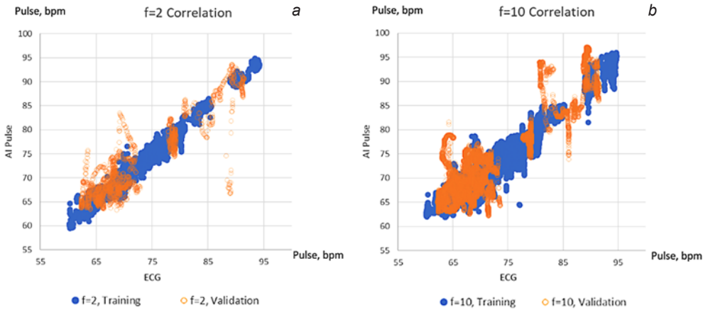
Fig. 4. Correlation dependence of HR measurement data of FVT+AI head MV analysis for the validation and training database for 2 Hz (a) and 10 Hz (b) on ECG data
